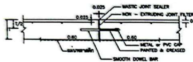
EXPANSION JOINT
