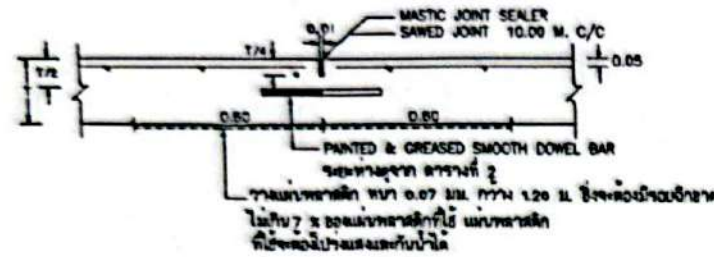
CONTRACTION JOINT
